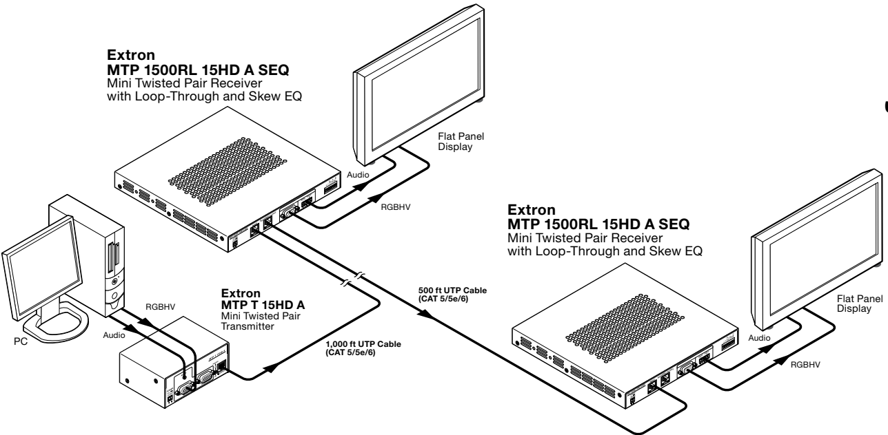
Figure 1 — Typical MTP 1500RL 15HD A SEQ application
