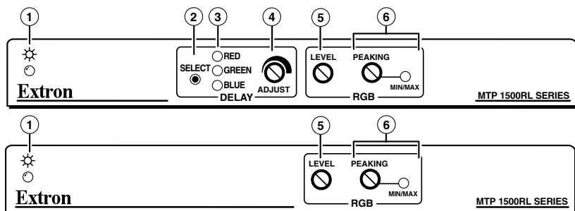
Figure 7 — MTP receiver series front panels
